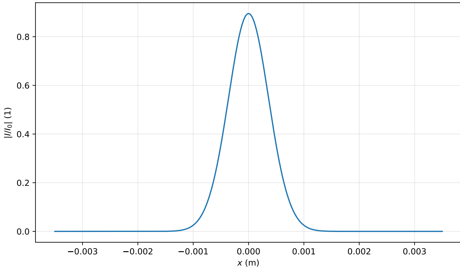
Intensity profile I(x, y = 0, z = 0.796m)/I_0 , P_{in}=0.1P_{cr} , artificial time
